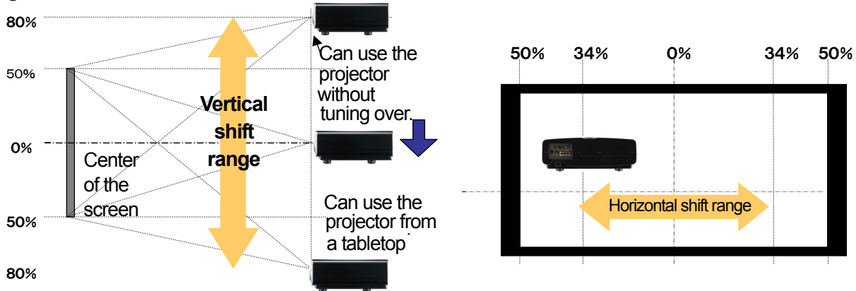
Figure 1. ±80% vertical, ±34% horizontal lens shift function
